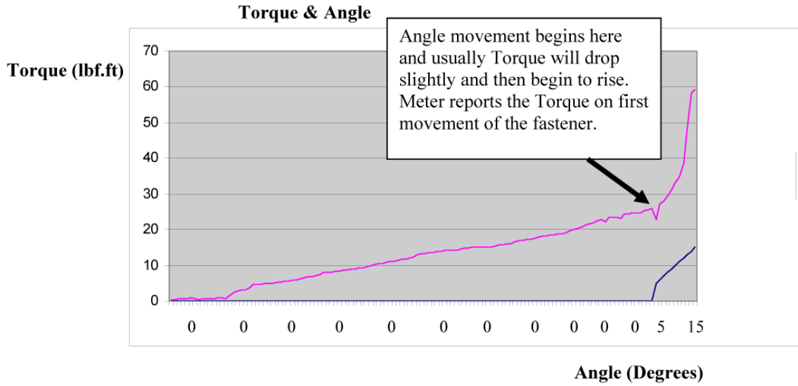
Exhibit #2 – Angular Movement of Bolt from a Minimum Value to a Nominal Value
